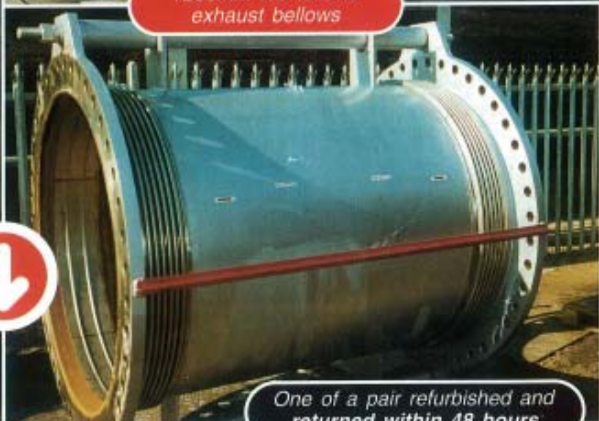
1200mm NB turbine exhaust bellows
